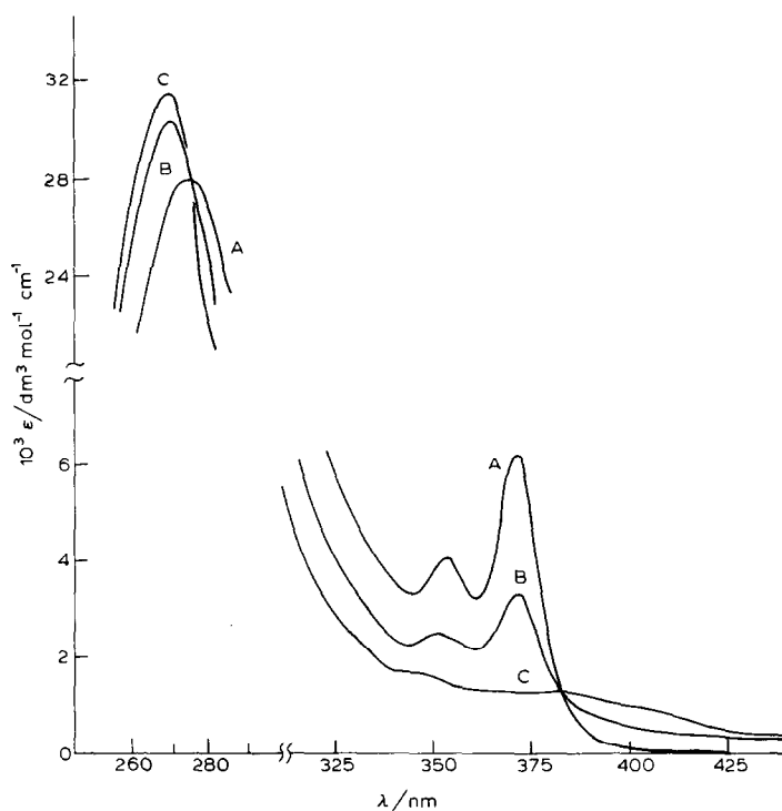
Fig. 10. UV-visible spectra of \text{Pt(phen)}_2^{2+} in water with added \text{CN}^- ion. Reprinted with permission from ref. 42.
