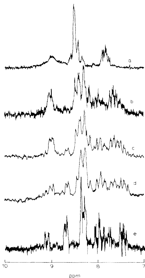
Fig. 9. 90 MHz ^1\text{H} NMR spectra of \text{Pt}(\text{bpy})_2^{2+} in (a) MeOH, (b) MeOH with [\text{MeO}^-] = \text{ca. } 0.1 \text{ M} immediately upon addition of the nucleophile, (c) reaction mixture after 10 min, (d) after 20 min, and (e) at the end of the reaction; temperature ca. 35^\circ\text{C} . Reprinted with permission from ref. 88.
